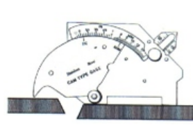
Misalignment (High-Low)
