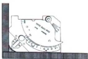
Fillet Weld Throat Size
