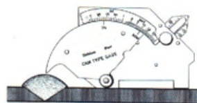
Excess Weld Metal (Capping Size)
