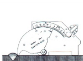
Depth of Undercut
